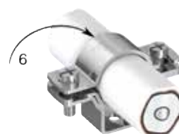
Screws in top part are self-retaining
