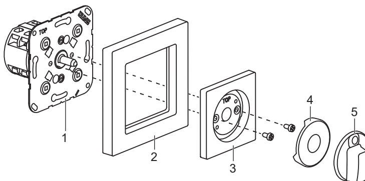
Fig. 1: Device components
