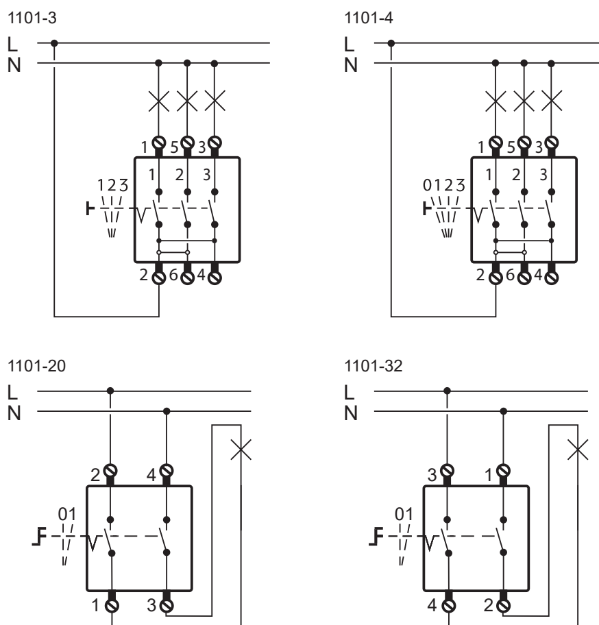
Fig. 2: Connection diagrams
