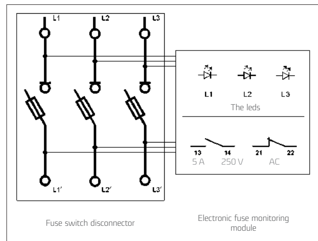
disconnecter contact position during normal operation
