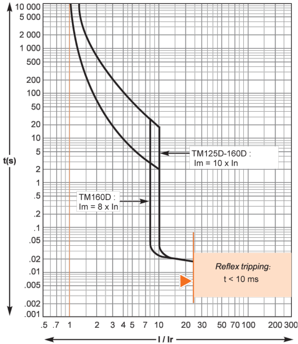
Performance Curves
